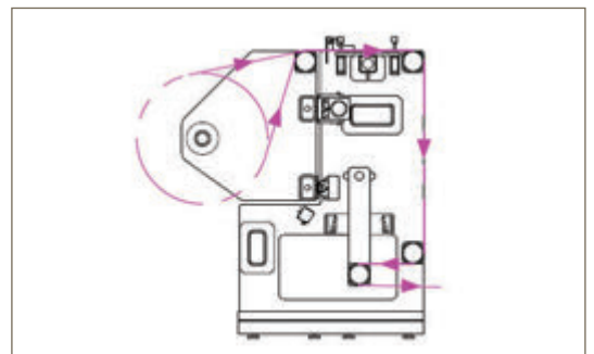
TYPICAL WEB PATH FOR SINGLE UNWIND STAND
