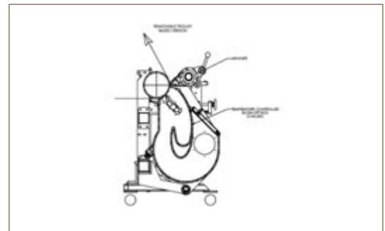
OPTIONAL TROLLEY BASED AIR KNIFE AND BLOW-OFF BOX
