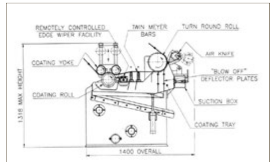
LINE DRAWING OF METERING ROD COATER WITH AIR KNIFE
